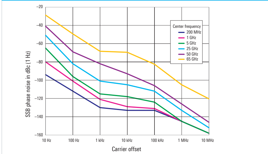
Phase noise of the R&S®FSU at various center frequencies
